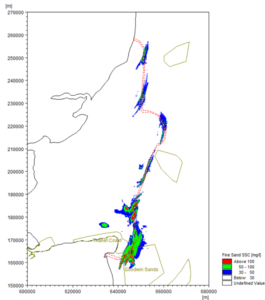
Plate 1.43. Maximum SSC levels over 14-day period for mud (left) and fine sand (right) for installation by jetting
