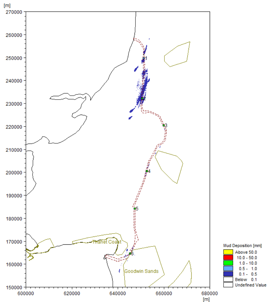
Plate 1.45. Maximum deposition over 14-day period for mud (left) and fine sand (right) for installation by jetting
