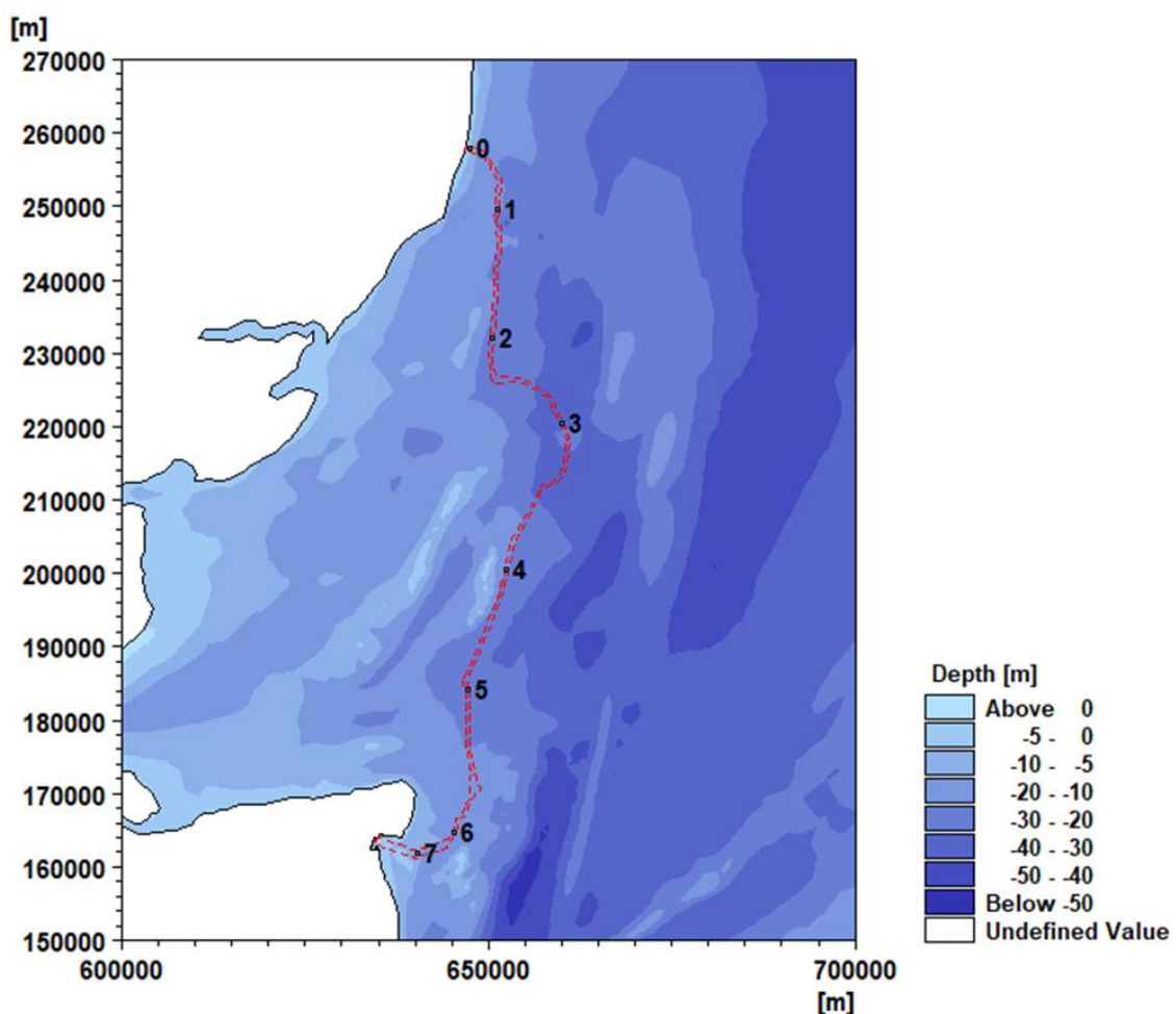
Plate 1.38 Hydrodynamic model bathymetry showing the Offshore Scheme Boundary (red line) and 8 sediment release locations
