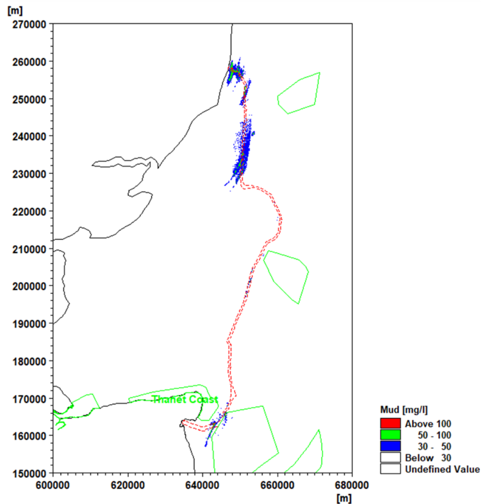
Plate 1.43. Maximum SSC levels over 14-day period for mud (left) and fine sand (right) for installation by jetting
