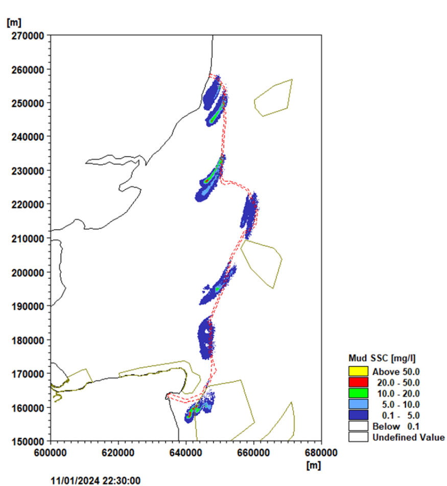
Plate 1.39 Mud SSC levels for jetting installation commencing on spring tides with output on flood (left) and ebb (right) tide after first 24 hours of activity. Note no mud in sample near Kent landfall, Point 7.
