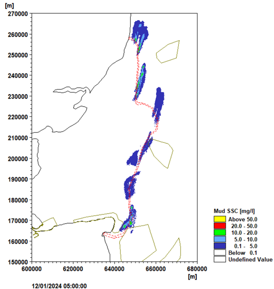
Plate 1.39 Mud SSC levels for jetting installation commencing on spring tides with output on flood (left) and ebb (right) tide after first 24 hours of activity. Note no mud in sample near Kent landfall, Point 7.
