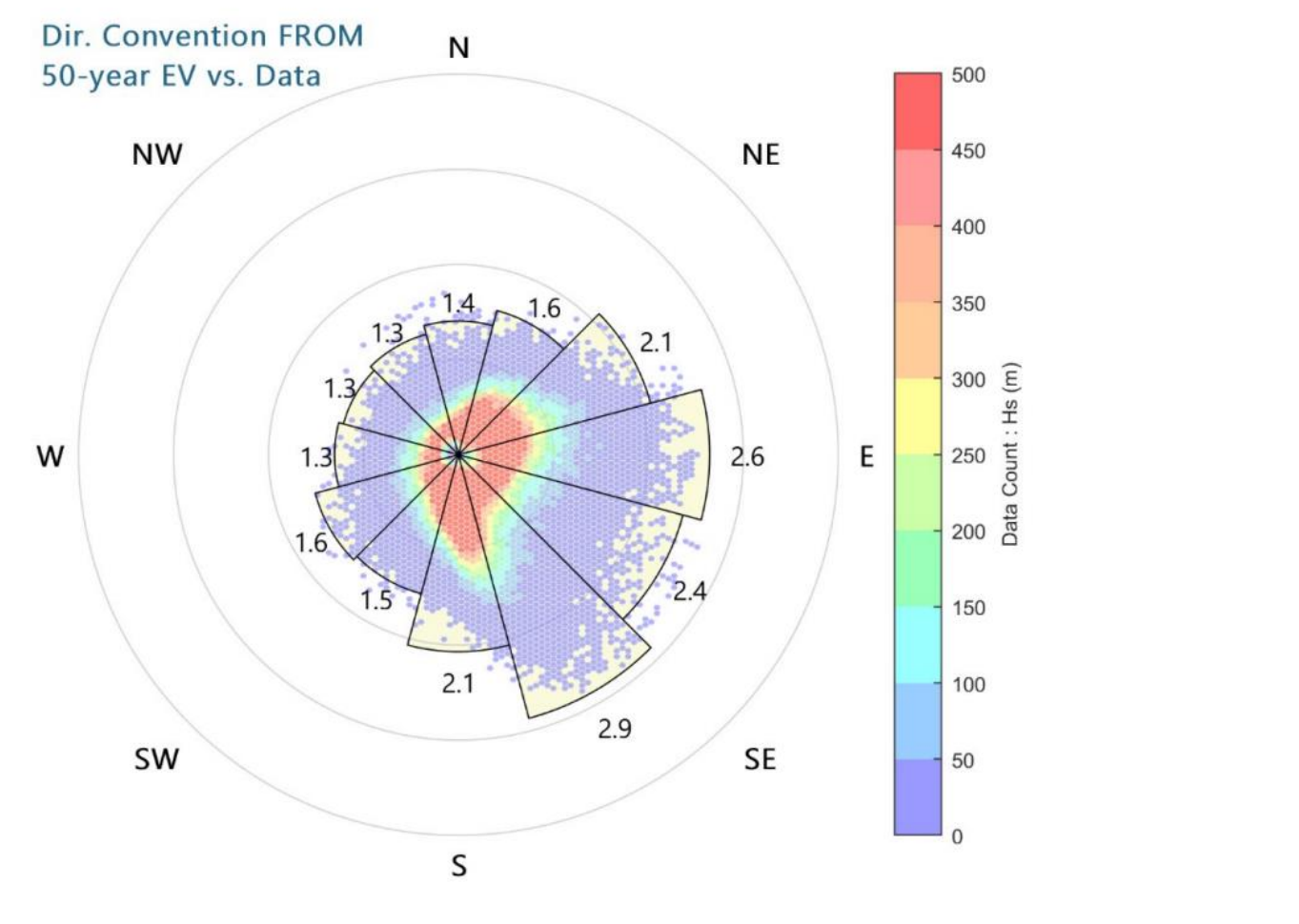
Plate 1.3 Wave rose of extreme wave heights at 1:50 return period for KP3, showing the amount of wave height data per sector and in black the extreme wave height per direction sector (ABPmer, 2024a).
